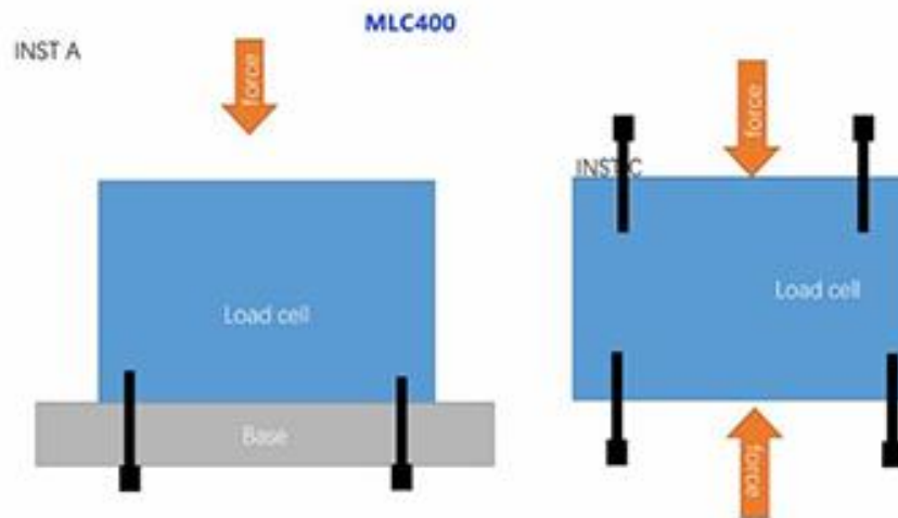
COMPRESSION LOAD CELL FORCE INSTALLATION
