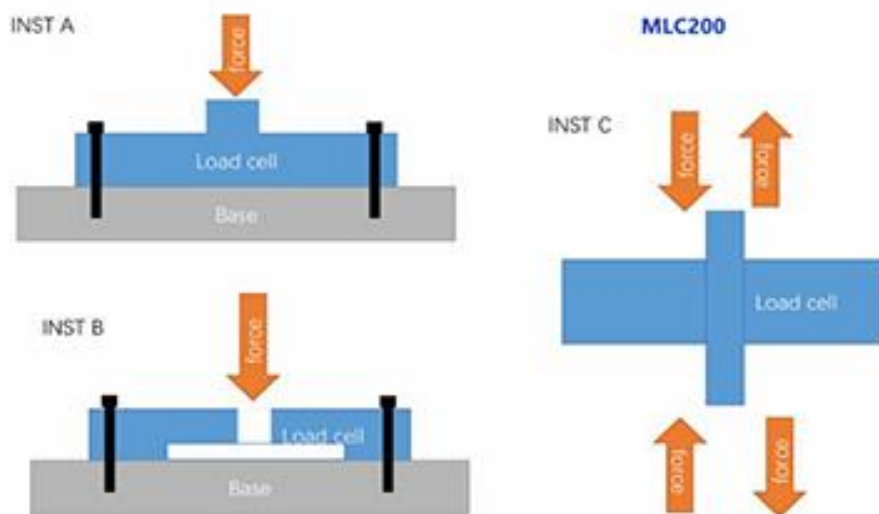
Round LOAD CELL FORCE INSTALLATION
